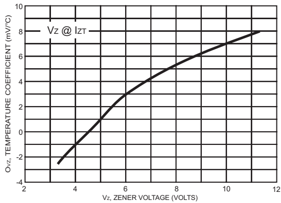
FIG.3- ZENER VOLTAGE - TO 12 VOLTS
