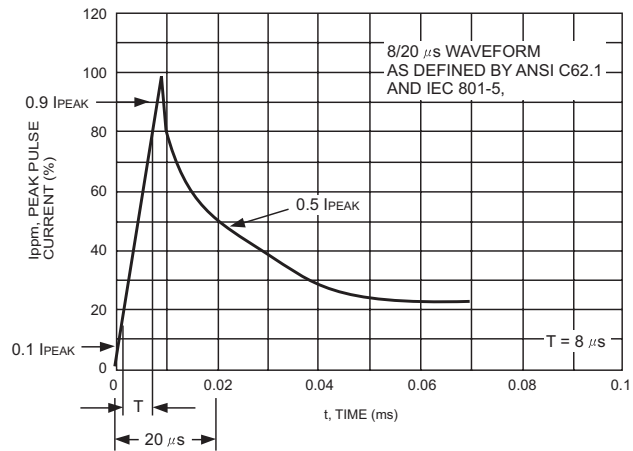
FIG.12- PULSE WAVEFORM
