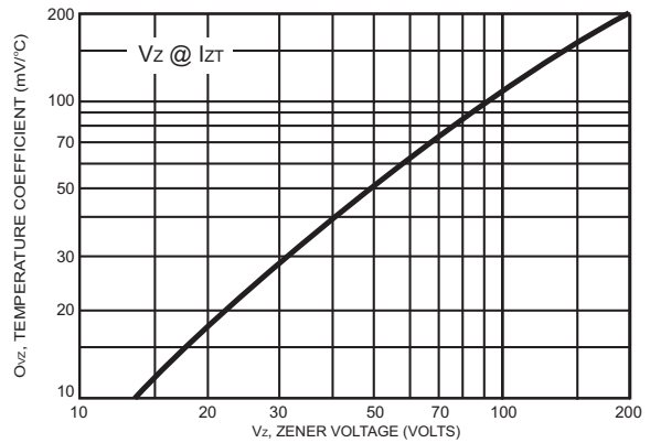
FIG.4- ZENER VOLTAGE - 14 TO 200 VOLTS
