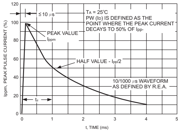
FIG.11- PULSE WAVEFORM
