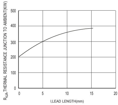
Figure2 Thermal Resistance vs Lead Length
