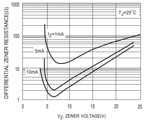
Figure4 Differential Zener Impedance
