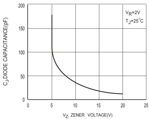
Figure3 Diode Capacitance vs Zener Voltage
