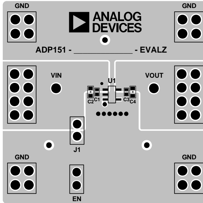
Figure 6. ADP151UJZ-RedyKit Evaluation Board Layout
