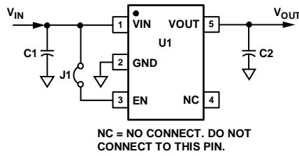
Figure 5. ADP151UJZ-RedyKit Evaluation Board Schematic
