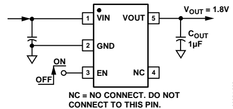
Figure 1. ADP151UJZ-RedyKit
