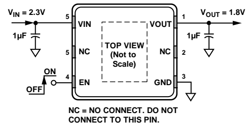
Figure 2. ADP151CPZ-RedyKit
