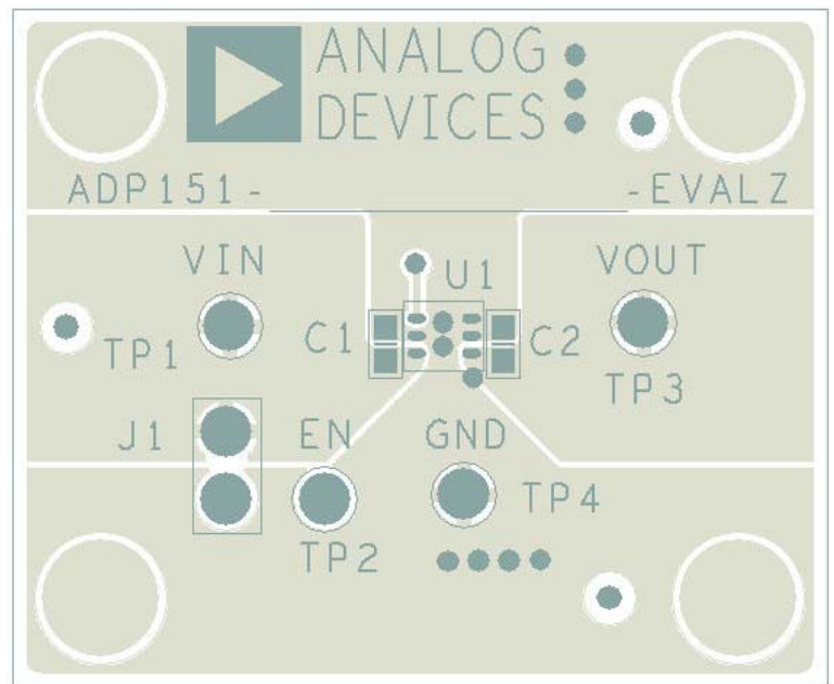
Figure 8. ADP151CPZ-RedyKit Evaluation Board Layout
