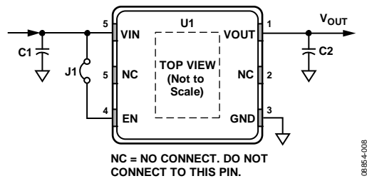
Figure 7. ADP151CPZ-RedyKit Evaluation Board Schematic
