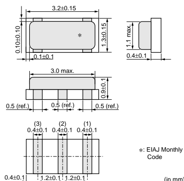
CSTCE_V_C 14.00-20.00MHz
