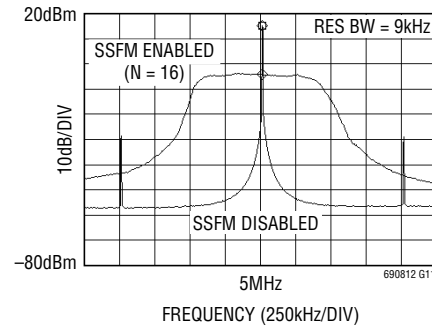
Output Frequency Spectrum with SSFM Enabled and Disabled
