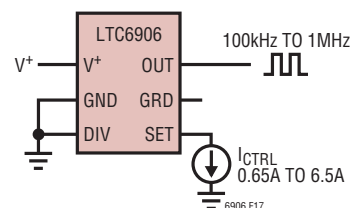
Figure 17. Current Controlled Oscillator
