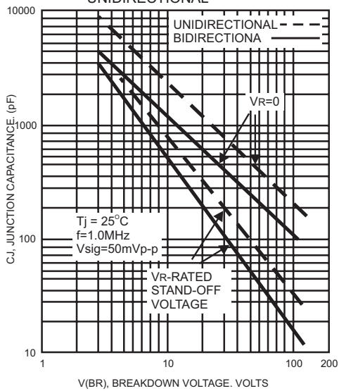
FIG.5- TYPICAL JUNCTION CAPACITANCE UNIDIRECTIONAL
