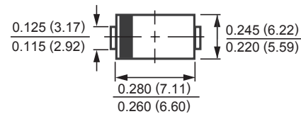
DO-214AB
