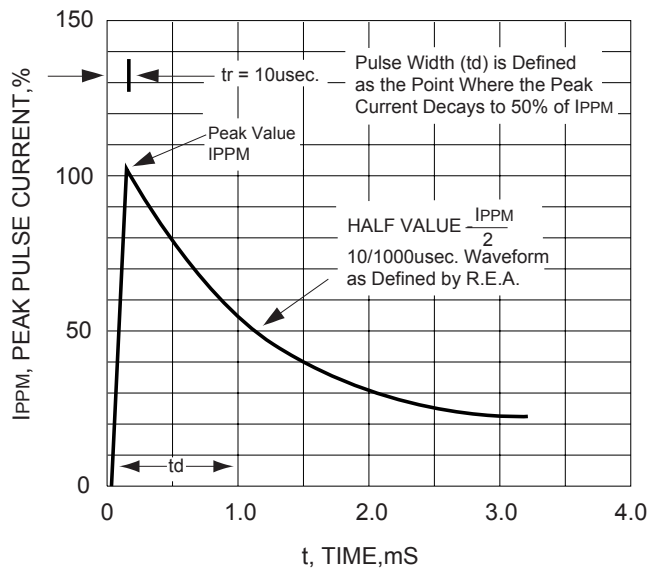
FIG. 3 - PULSE WAVEFORM
