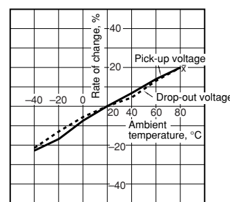
9. Ambient temperature characteristics Tested sample: TQ2SA-12V, 5 pcs.
