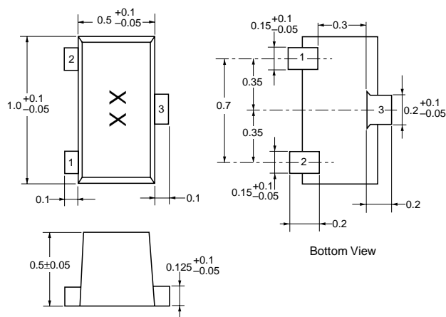
PACKAGE OUTLINE M13
