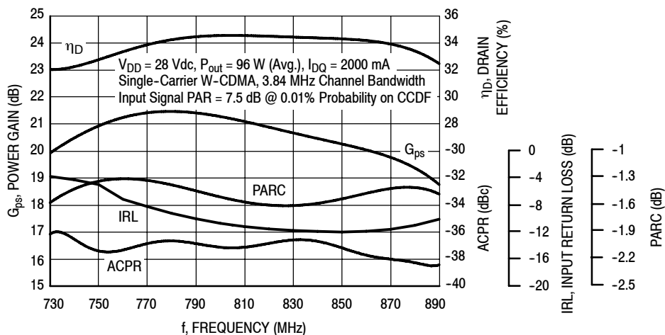
Figure 4. Output Peak-to-Average Ratio Compression (PARC) Broadband Performance @ P out = 96 Watts Avg.
