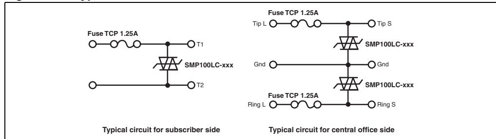
Figure 10. Typical circuits
