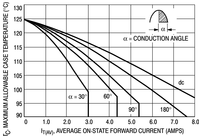
Figure 1. Current Derating
