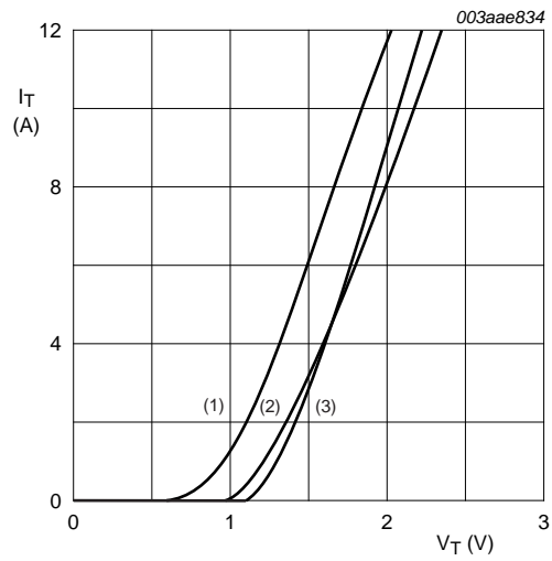
V_o = 1.27\text{ V} R_s = 0.091\ \Omega (1) T_j = 125^\circ\text{C} ; typical values (2) T_j = 125^\circ\text{C} ; maximum values (3) T_j = 25^\circ\text{C} ; maximum values Fig 10. On-state current as a function of on-state voltage
