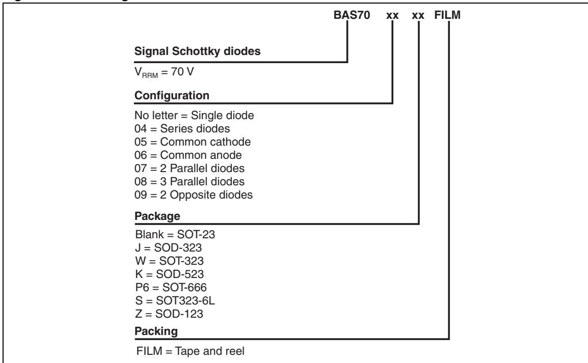
Figure 15. Ordering information scheme
