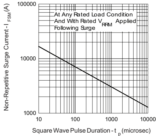
Fig. 7 - Maximum Non-Repitative Surge Current
