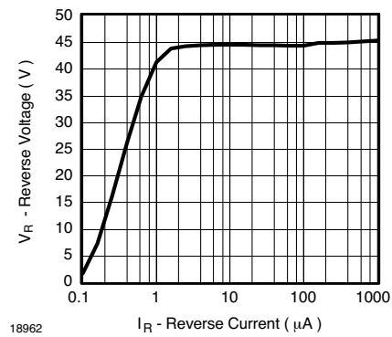
Figure 3. Typical Reverse Voltage vs. Reverse Current
