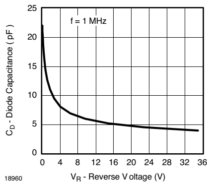
Figure 1. Typical Capacitance vs. Reverse Voltage
