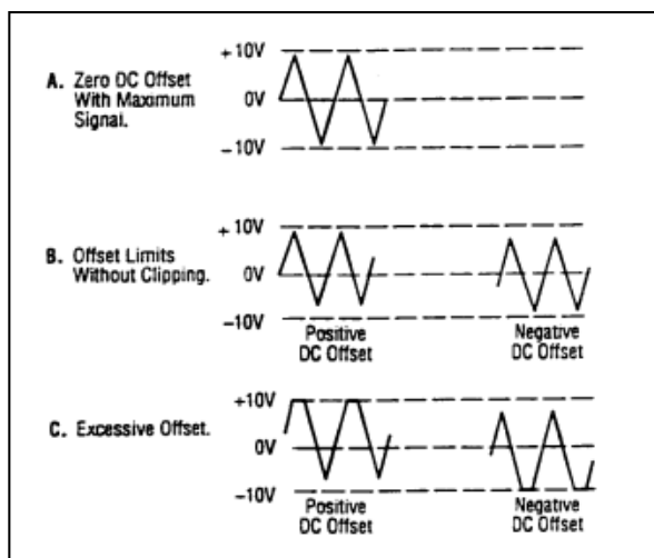
Figure 3. Use of DC OFFSET Control
