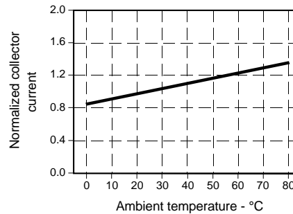
Collector Current vs Ambient Temperature
