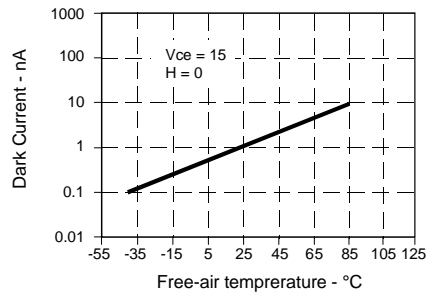
Dark Current vs Temperature
