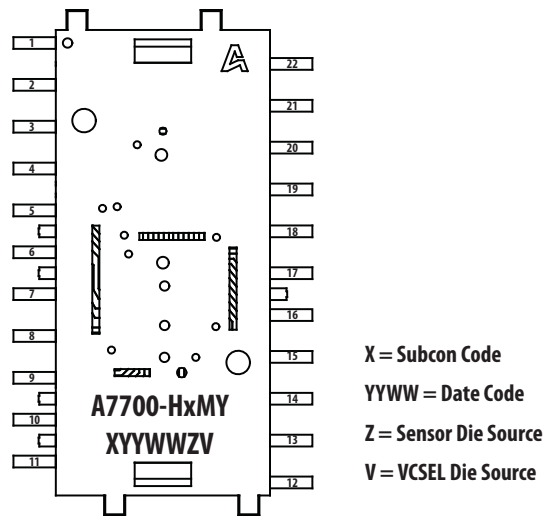
Figure 1. Device Pinout
