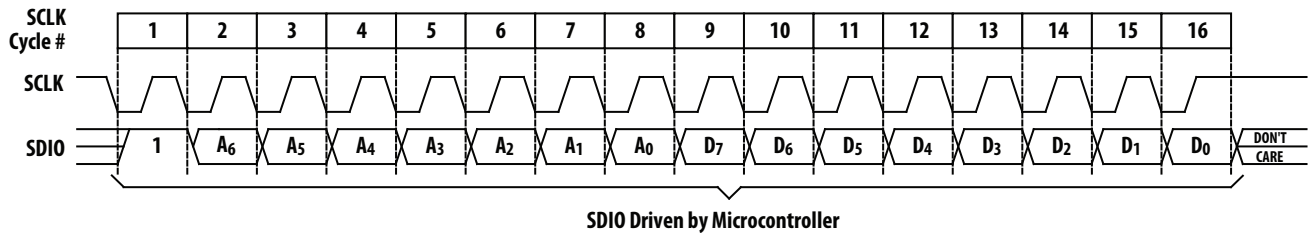
Figure 16. Write operation
