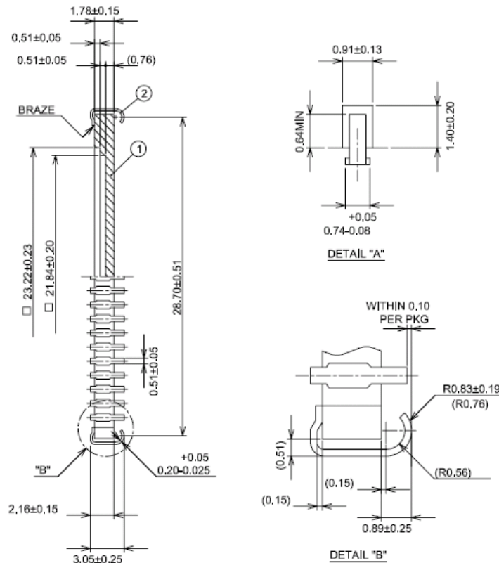
Figure 2. Physical and Geometrical Package Drawings
