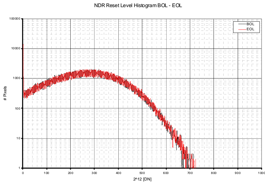
Figure 15. FPN Histogram in NDR before and after 2000h Life test
