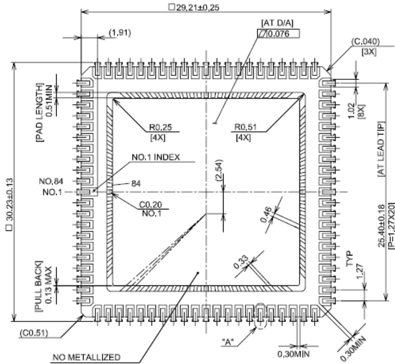
Figure 2. Physical and Geometrical Package Drawings
