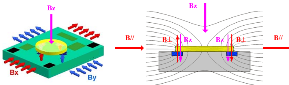
Figure 4 - Tria \otimes is™ sensor front-end (4 Hall plates + IMC® disk)
