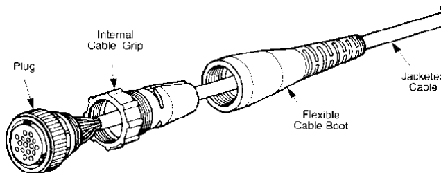
Internal Cable Grip
