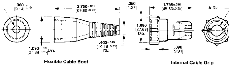
Internal Cable Grip
