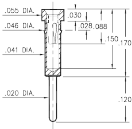
0462-0-15-XX-X1-XX-04-0 Press-fit in .043 mounting hole
