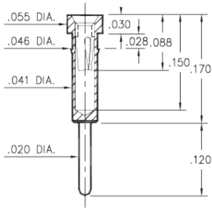
0462-0-15-XX-X1-XX-04-0 Press-fit in .043 mounting hole
