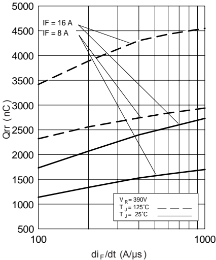
Fig. 10 - Typical Stored Charge vs. di_F/dt
