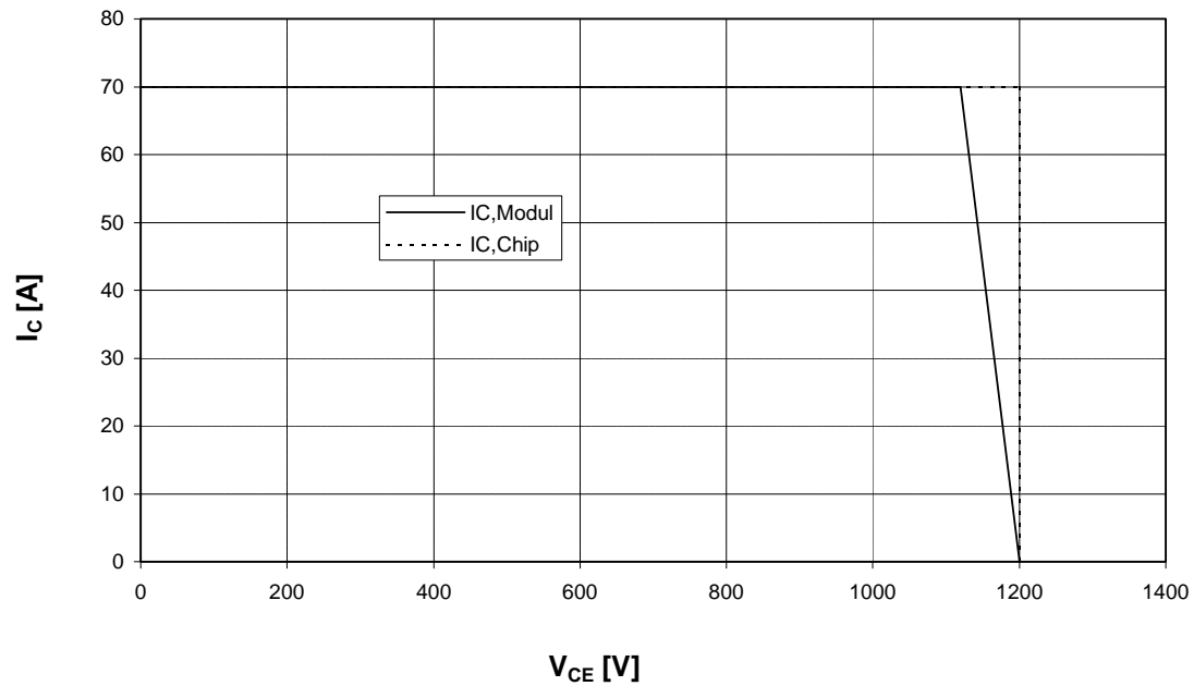
Sicherer Arbeitsbereich Wechselr. (RBSOA) I_C = f(V_{CE}) Reverse bias safe operating area Inverter (RBSOA) T_{vi} = 125^\circ\text{C}, V_{GE} = \pm 15\text{V}, R_G = 22 \text{ Ohm}
