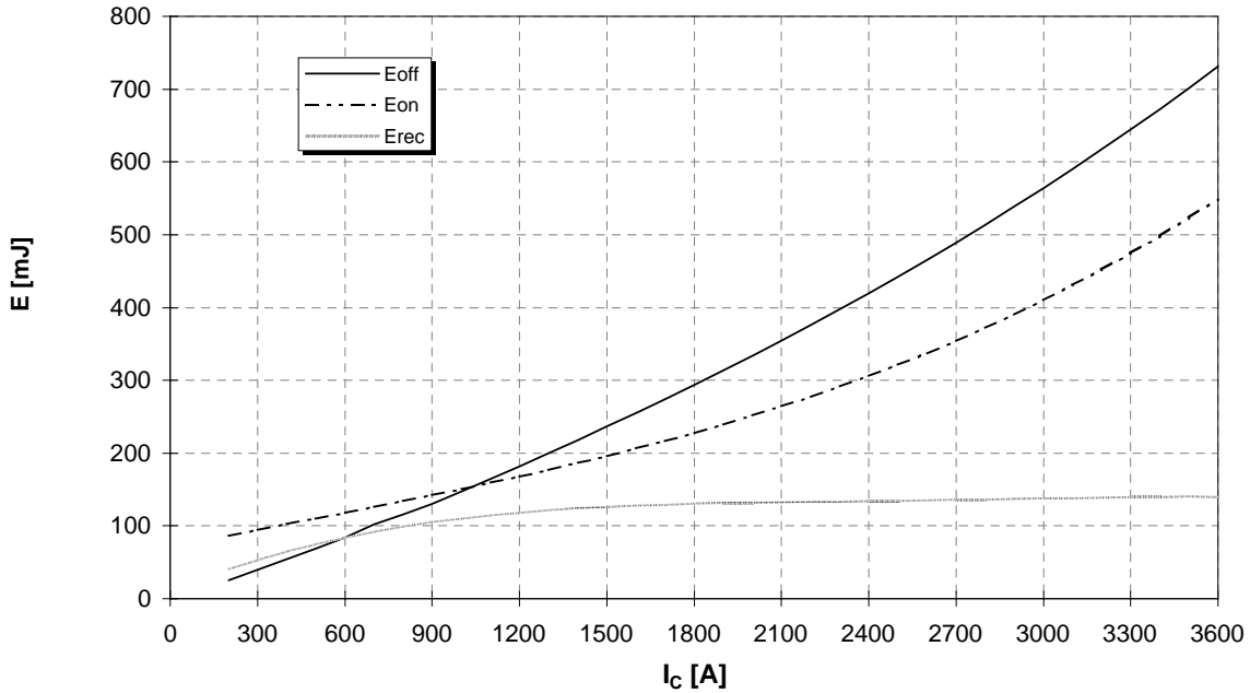
Schaltverluste (typisch) E_{on} = f(I_C) , E_{off} = f(I_C) , E_{rec} = f(I_C) Switching losses (typical) V_{GE} = \pm 15V , R_{gon} = R_{goff} = 0,51 \Omega , V_{CE} = 600V , T_j = 125^\circ C
