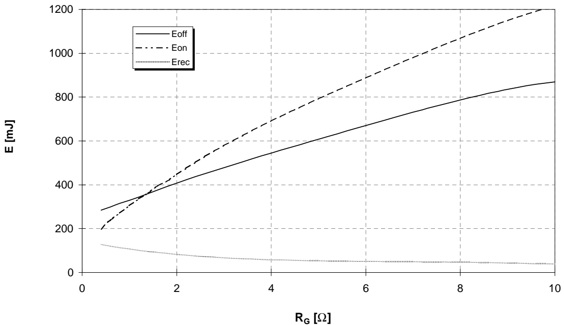
Schaltverluste (typisch) E_{on} = f(R_G) , E_{off} = f(R_G) , E_{rec} = f(R_G) Switching losses (typical) V_{GE} = \pm 15V , I_C = 1800A , V_{CE} = 600V , T_j = 125^\circ C
