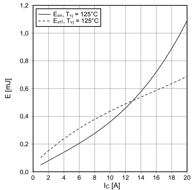
Schaltverluste IGBT-Wechselr. (typisch) switching losses IGBT-inverter (typical) E_{on} = f(I_c) , E_{off} = f(I_c) V_{GE} = \pm 15\text{ V} , R_{Gon} = 82\ \Omega , R_{Goff} = 82\ \Omega , V_{CE} = 300\text{ V}
