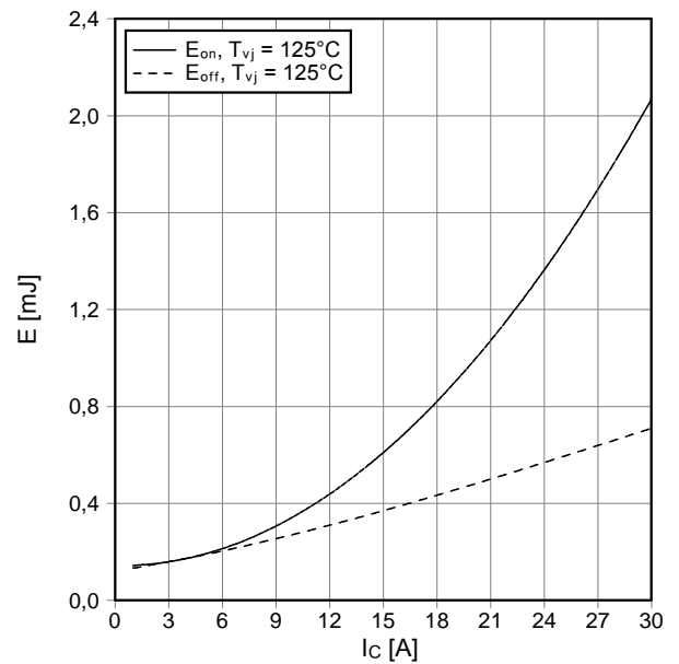
Schaltverluste IGBT-Wechselr. (typisch) switching losses IGBT-inverter (typical) E_{on} = f(I_c) , E_{off} = f(I_c) V_{GE} = \pm 15\text{ V} , R_{Gon} = 68\ \Omega , R_{Goff} = 68\ \Omega , V_{CE} = 300\text{ V}
