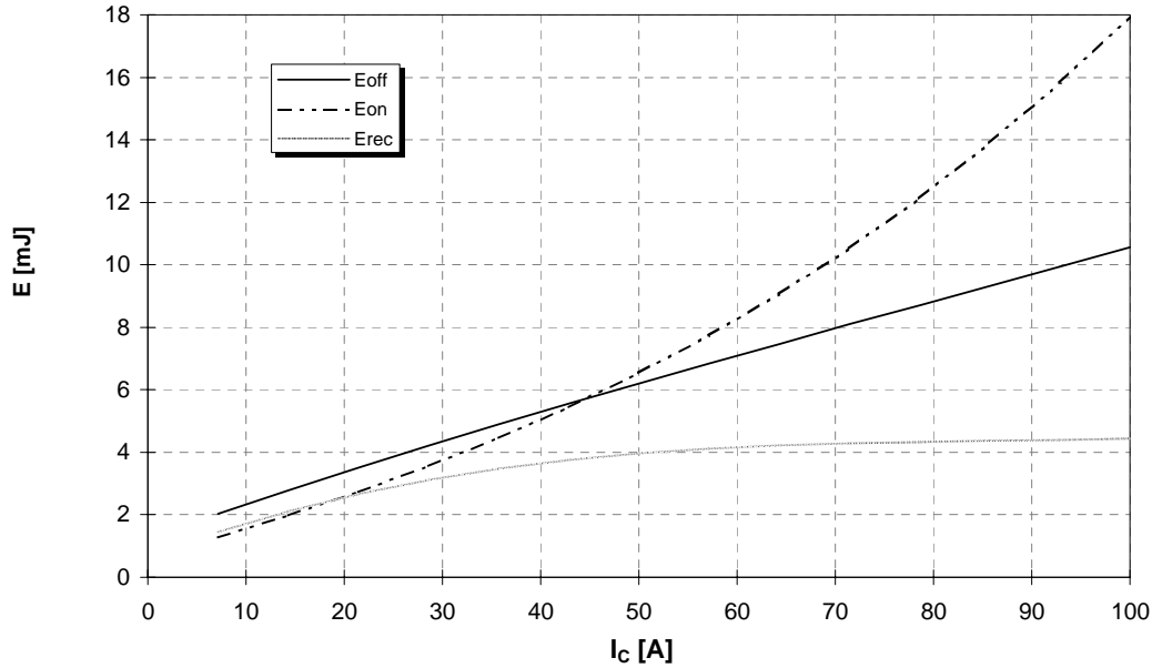
Schaltverluste (typisch) E_{on} = f(I_c) , E_{off} = f(I_c) , E_{rec} = f(I_c) Switching losses (typical) V_{GE}=15V , R_{gon} = R_{goff} = 15 \Omega , V_{CE} = 600V , T_j = 125^\circ C
