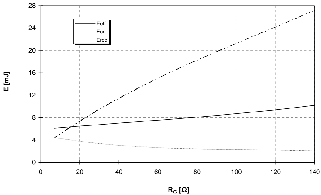
Schaltverluste (typisch) E_{on} = f(R_G) , E_{off} = f(R_G) , E_{rec} = f(R_G) Switching losses (typical) V_{GE}=15V , I_c = 50A , V_{CE} = 600V , T_j = 125^\circ C
