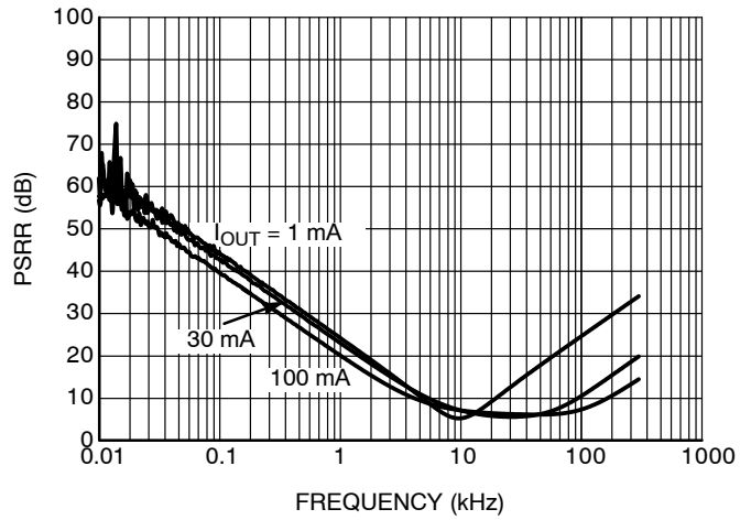
Figure 18. PSRR, 5.0 V Version, V_{IN} = 8.0 V
