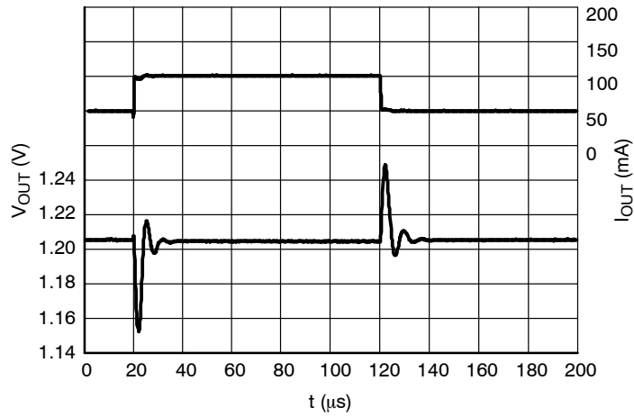
Figure 26. Load Transients, 3.0 V Version, I_{\text{OUT}} = 1 - 20 \text{ mA} , t_{\text{R}} = t_{\text{F}} = 50 \mu\text{s} , V_{\text{IN}} = 6.0 \text{ V}
