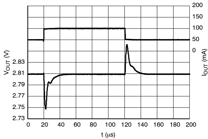
Figure 27. Load Transients, 5.0 V Version, I_{\text{OUT}} = 1 - 20 \text{ mA} , t_{\text{R}} = t_{\text{F}} = 50 \mu\text{s} , V_{\text{IN}} = 8.0 \text{ V}
