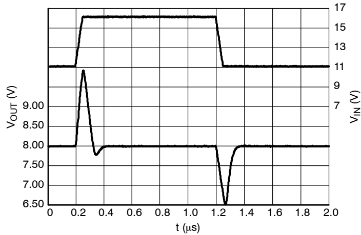
Figure 25. Line Transients, 8.0 V Version, t_{\text{R}} = t_{\text{F}} = 5 \mu\text{s} , I_{\text{OUT}} = 1 \text{ mA}
