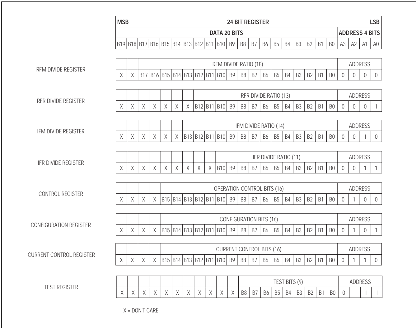
Figure 1. Register Configuration
