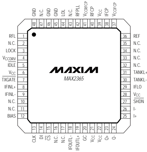
(T) QFN-EP
