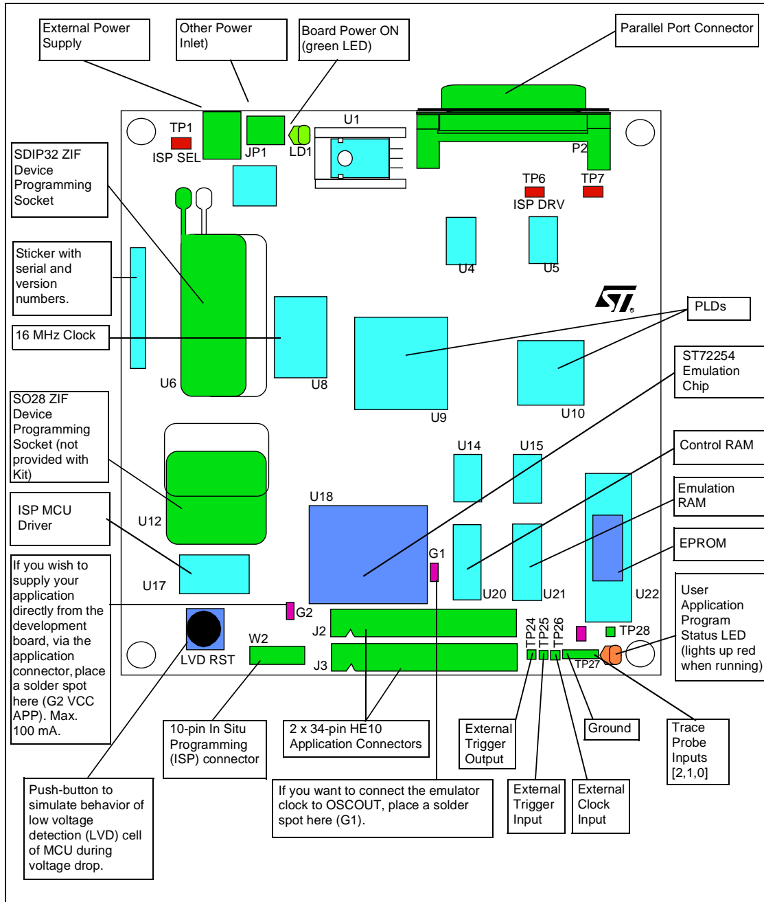
Figure 4: Development board layout
