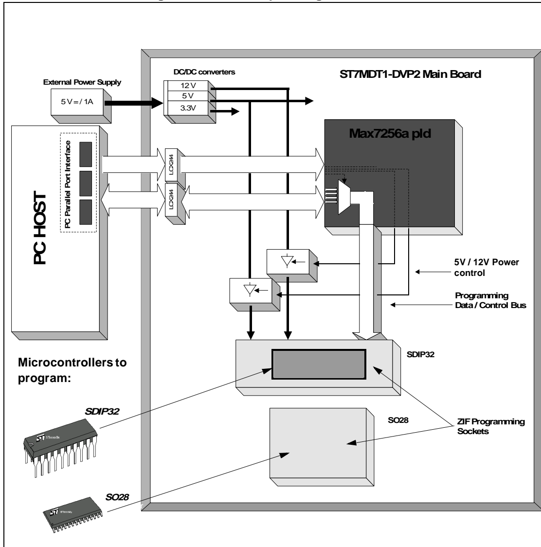
Figure 7: General eproming architecture
