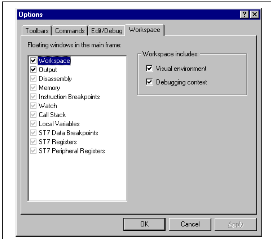
Figure 5: Options window
