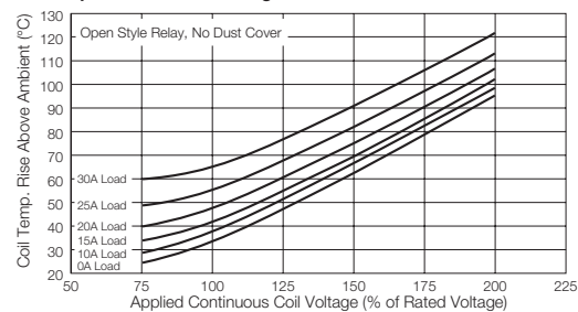
Ambient temperature vs. coil voltage – 1W coil
