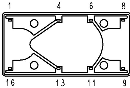
Relay - bottom view
