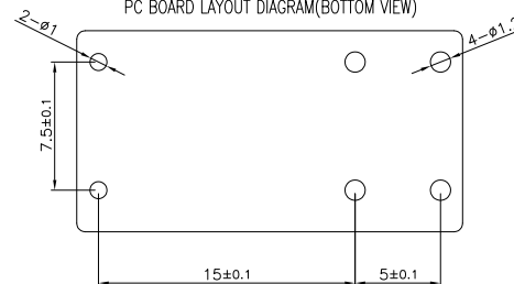
PC BOARD LAYOUT DIAGRAM(BOTTOM VIEW)
