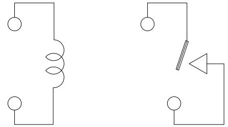
CONNECTION FIGURE
