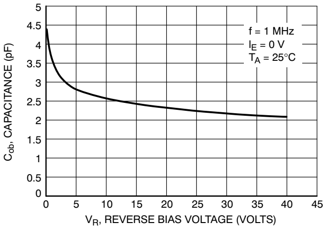
Figure 49. Output Capacitance
