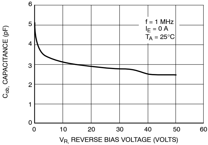
Figure 44. Output Capacitance
