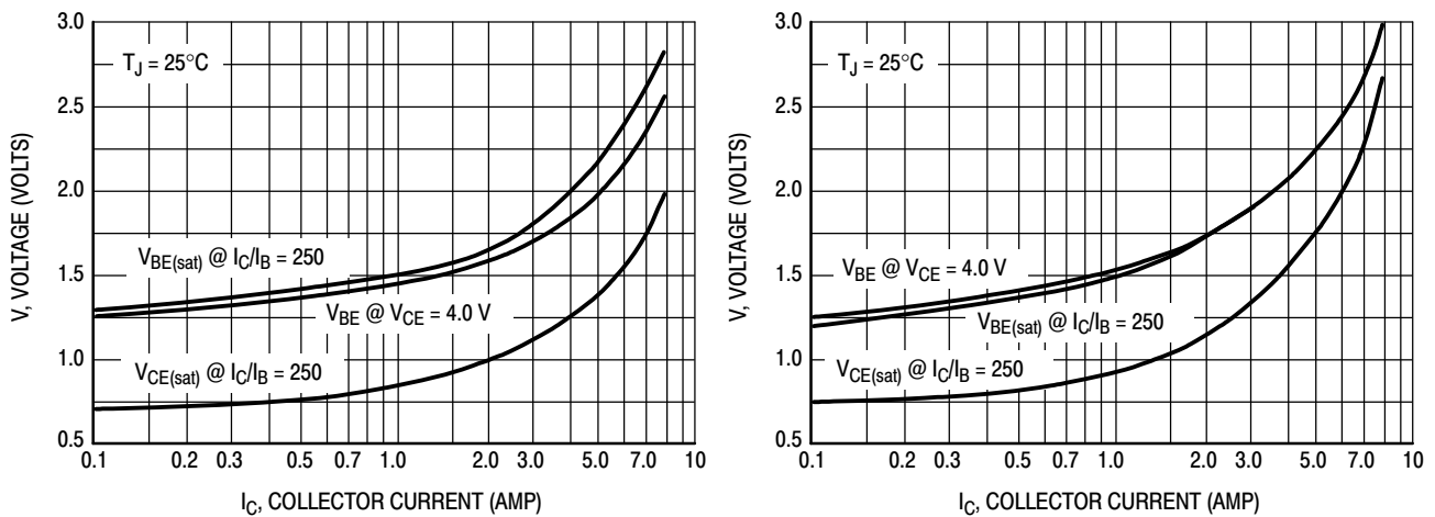
Figure 10. "On" Voltages
