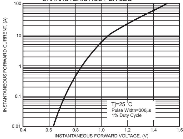
FIG.5- TYPICAL FORWARD VOLTAGE CHARACTERISTICS PER LEG
