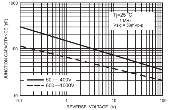
FIG.4- TYPICAL JUNCTION CAPACITANCE PER LEG
