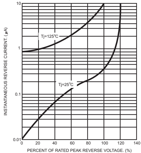
FIG.5- TYPICAL REVERSE CHARACTERISTICS PER BRIDGE ELEMENT
