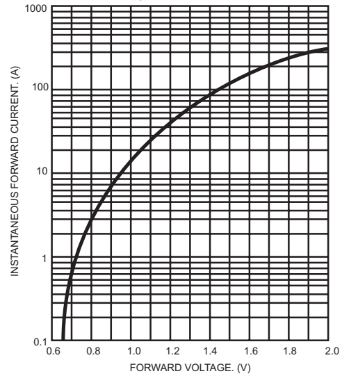
FIG.2- TYPICAL FORWARD CHARACTERISTICS PER BRIDGE ELEMENT
