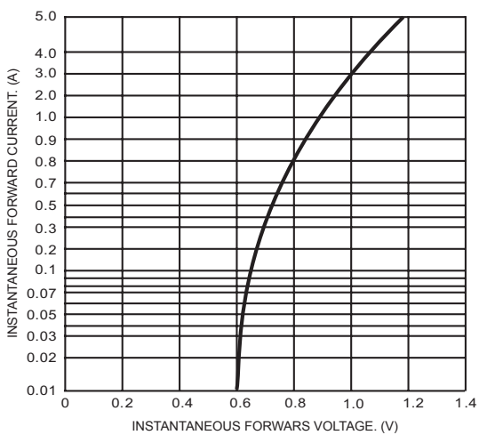
FIG.5-TYPICAL FORWARD CHARACTERISTICS
