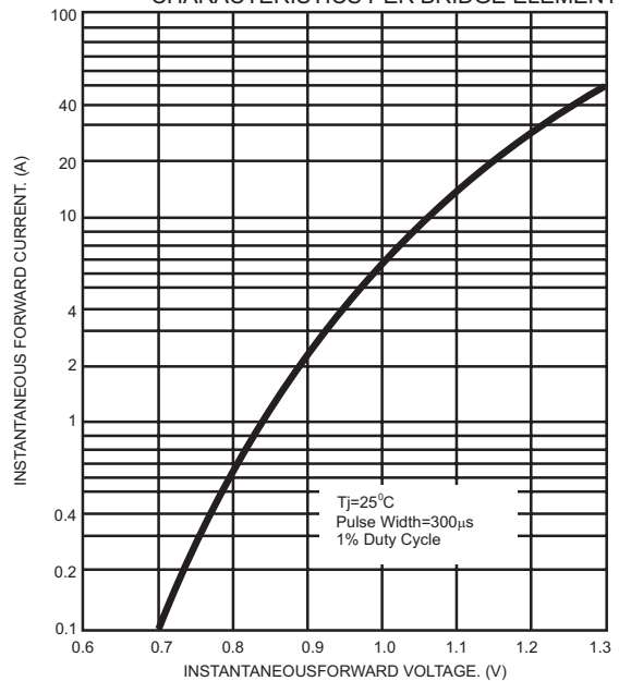
FIG.5- TYPICAL INSTANTANEOUS FORWARD CHARACTERISTICS PER BRIDGE ELEMENT
