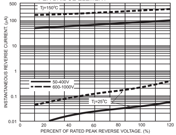
FIG.2- TYPICAL REVERSE CHARACTERISTICS PER BRIDGE ELEMENT
