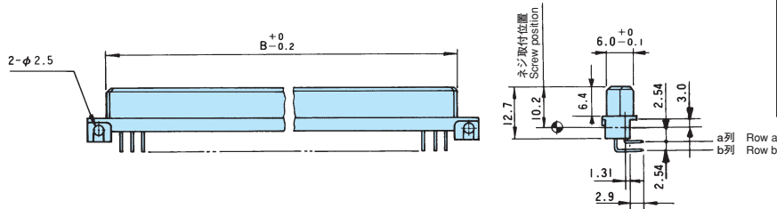
推奨取付寸法 Recommended mounting dimensions
