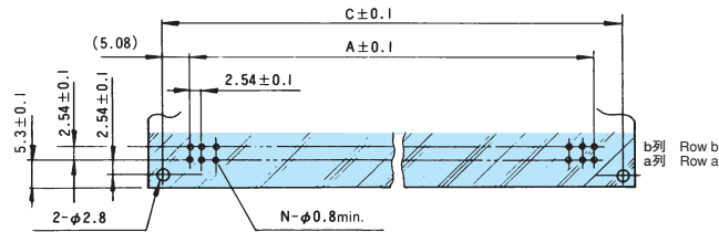
推奨取付寸法 Recommended mounting dimensions
