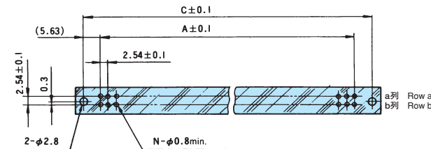
推奨取付寸法 Recommended mounting dimensions
