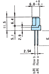
推奨取付寸法 Recommended mounting dimensions
