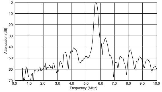
SFSRA5M74BF00-B0
