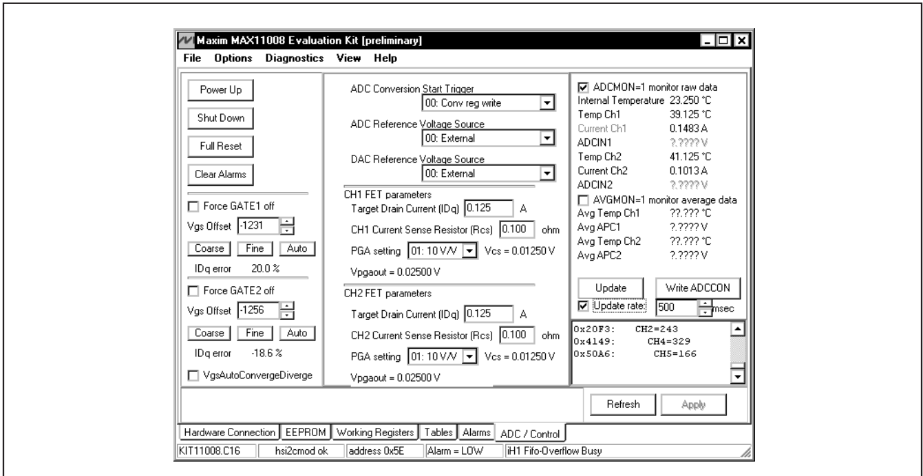
Figure 6. ADC / Control Tab Showing a Typical Configuration
